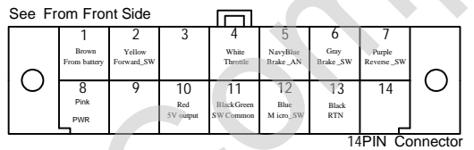
Dual PM/PMB/PMH Controller Assembly Wiring Diagram
